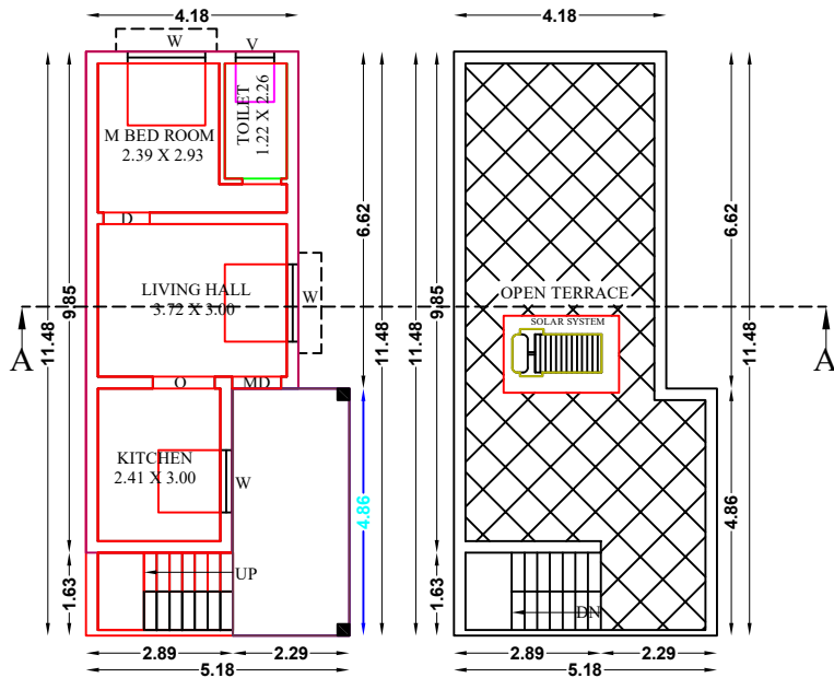
FLOOR - GROUND GROUND FLOOR PLAN
