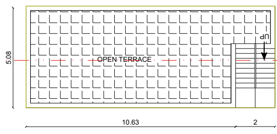
FLOOR - TERRACE PRO.TERRACE FLOOR PLAN
