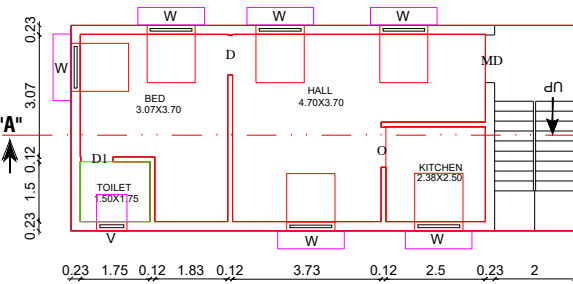
FLOOR - GROUND PRO.GROUND FLOOR PLAN
