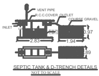
SEPTIC TANK & D-TRENCH DETAILS NOT TO SCALE
