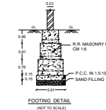
FOUNDATION DETAIL (NOT TO SCALE)
