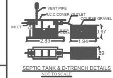
SEPTIC TANK & D-TRENCH DETAILS NOT TO SCALE
