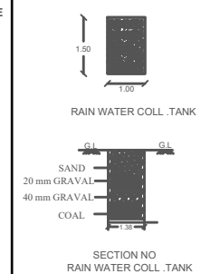
SECTION NO RAIN WATER COLL. TANK
