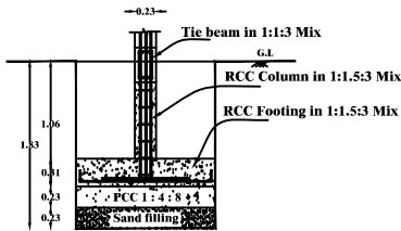
CROSS SECTION ON 'C - C'
