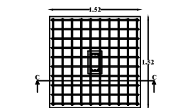
PLAN COLOUMN FOUNDATION DETAILS
