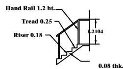
STAIRCASE DETAILS
