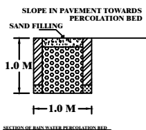
SECTION OF RAIN WATER PERCOLATION BED
