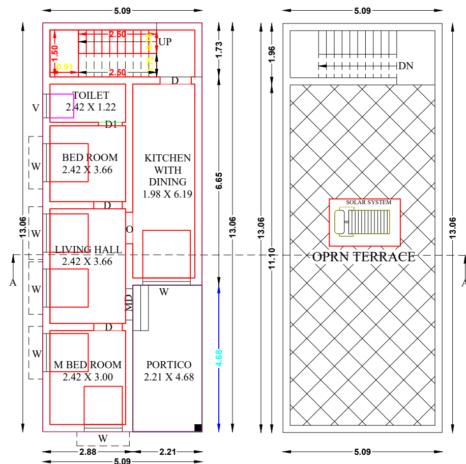
FLOOR - GROUND GROUND FLOOR PLAN
