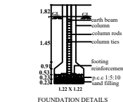
FOUNDATION DETAILS
