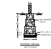
SEPTIC TANK & D-TRENCH DETAILS
