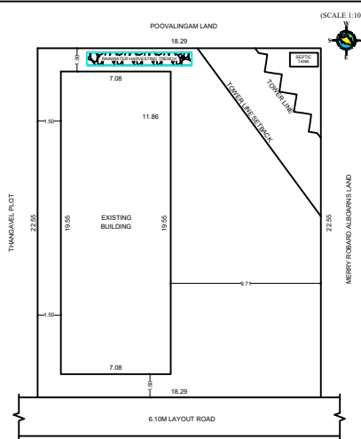
SITE PLAN (EXISTING)
