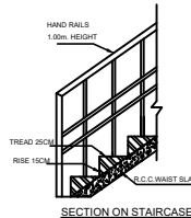
SECTION ON STAIRCASE
