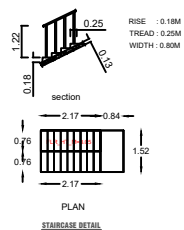
STAIRCASE DETAIL
