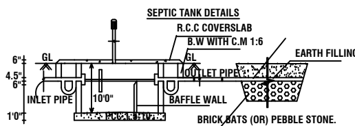
SEPTIC TANK DETAILS
