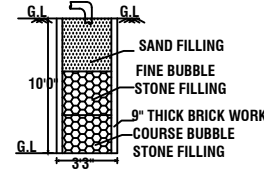
SECTION ON RAIN WATER COLLECTION TANK
