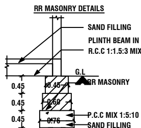
RR MASONRY DETAILS
