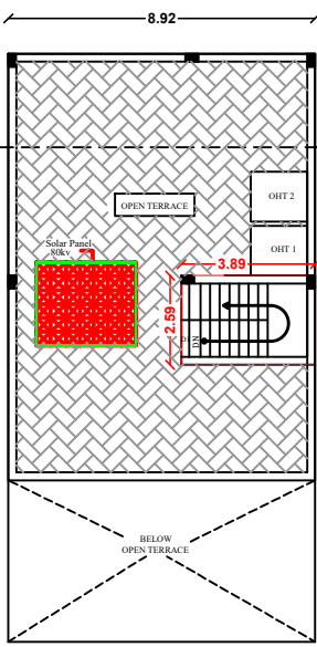
PRO.TERRACE FLOOR PLAN
