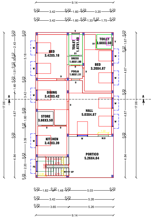
FLOOR-GROUND PRO.GROUND FLOOR PLAN
