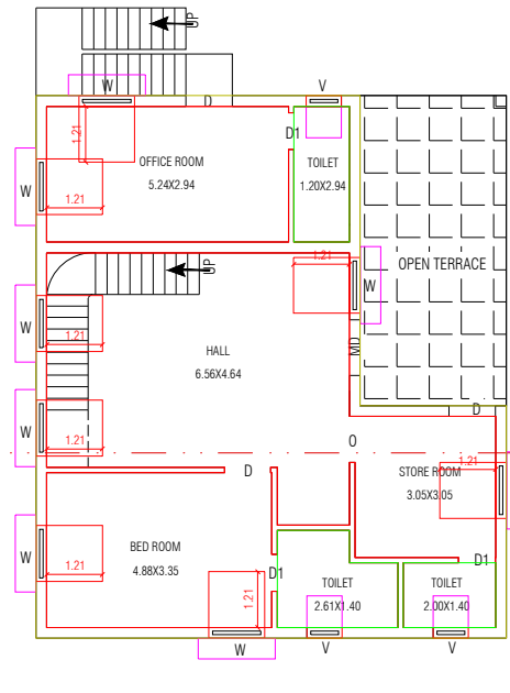
FLOOR - FIRST PRO.FIRST FLOOR PLAN
