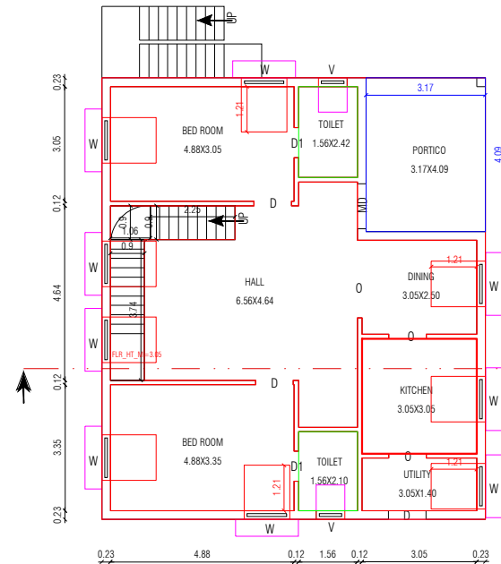
FLOOR - GROUND PRO.GROUND FLOOR PLAN
