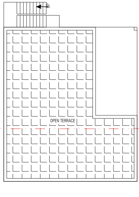
FLOOR - TERRACE PRO.TERRACE FLOOR PLAN
