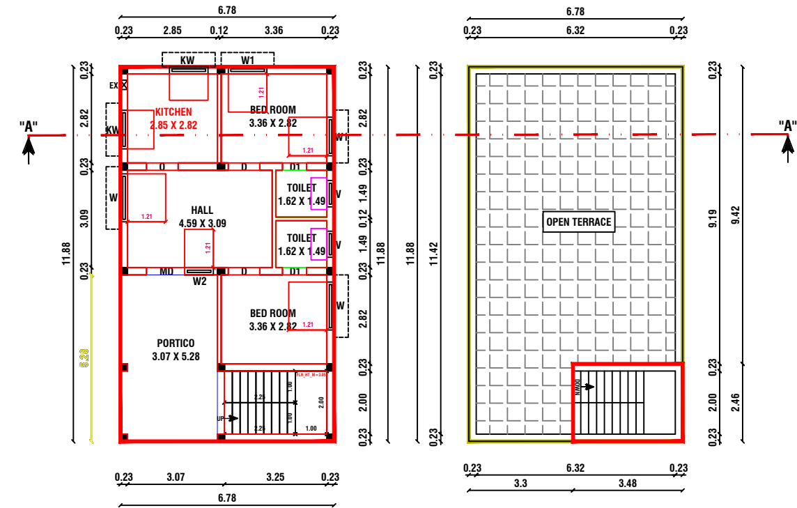
FLOOR - GROUND PRO. GROUND FLOOR PLAN FLOOR - TERRACE PRO. TERRACE FLOOR PLAN
