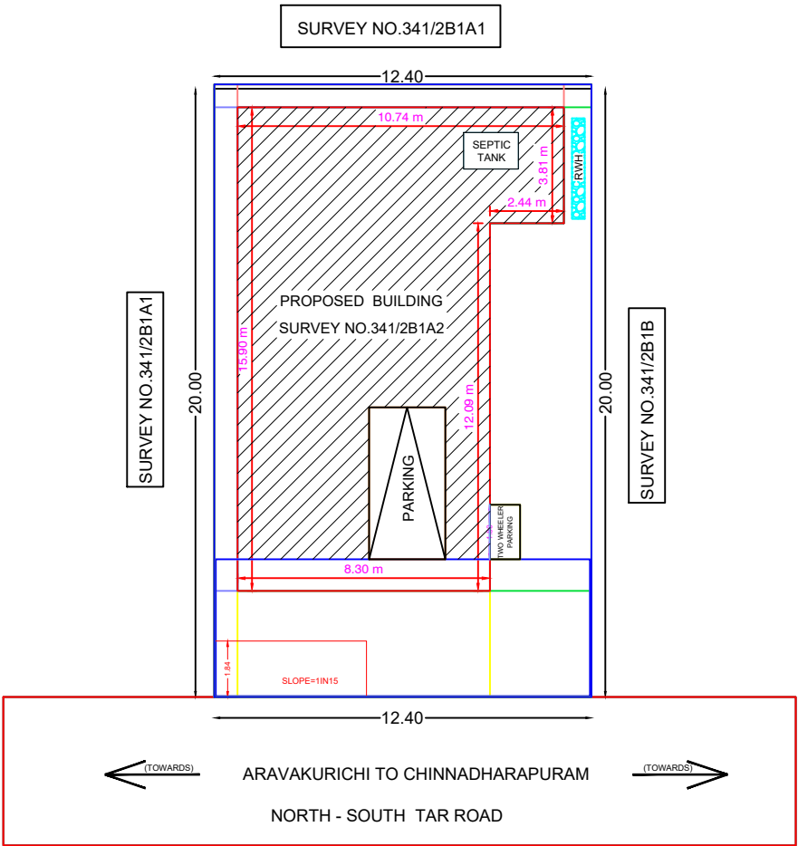
SITE PLAN
