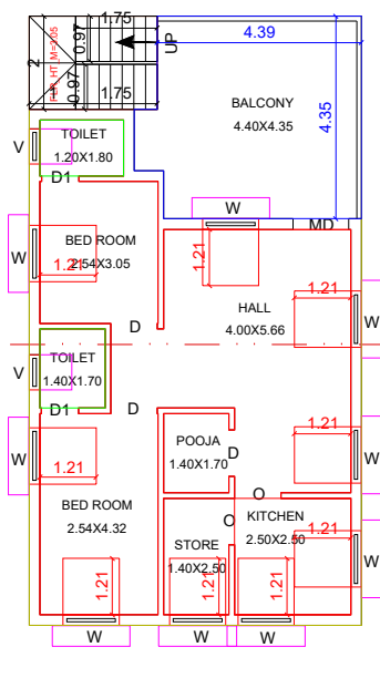
FLOOR - SECOND PRO.SECOND FLOOR PLAN
