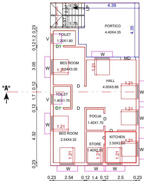
FLOOR - GROUND EXT.GROUND FLOOR PLAN
