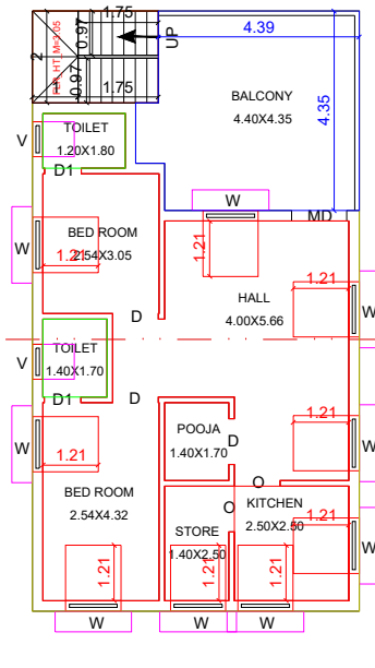
FLOOR - FIRST EXT.FIRST FLOOR PLAN
