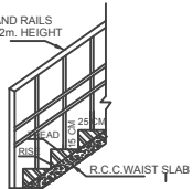
SECTION ON STAIRCASE
