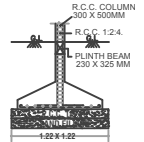
FOUNDATION DETAIL (NOT TO SCALE)
