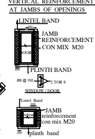
VERTICAL REINFORCEMENT AT JAMBS OF OPENINGS
