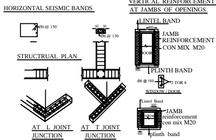
VERTICAL REINFORCEMENT AT JAMBS OF OPENINGS
