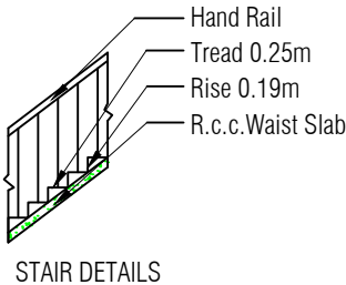
STAIR DETAILS
