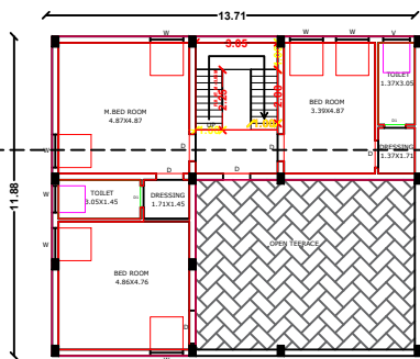
FLOOR - FIRST PRO. FIRST FLOOR PLAN
