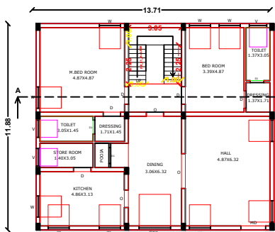
FLOOR - GROUND PRO. GROUND FLOOR PLAN
