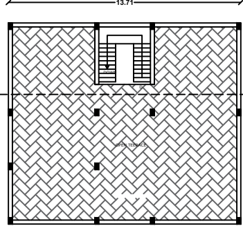
FLOOR - TERRACE PRO. TERRACE FLOOR PLAN
