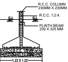
FOUNDATION DETAIL (NOT TO SCALE)
