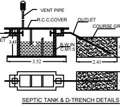
SEPTIC TANK & D-TRENCH DETAILS
