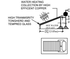
SOLAR HOT WATER SYSTEM DETAIL NOT TO SCALE
