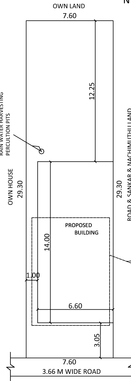
SITE PLAN
