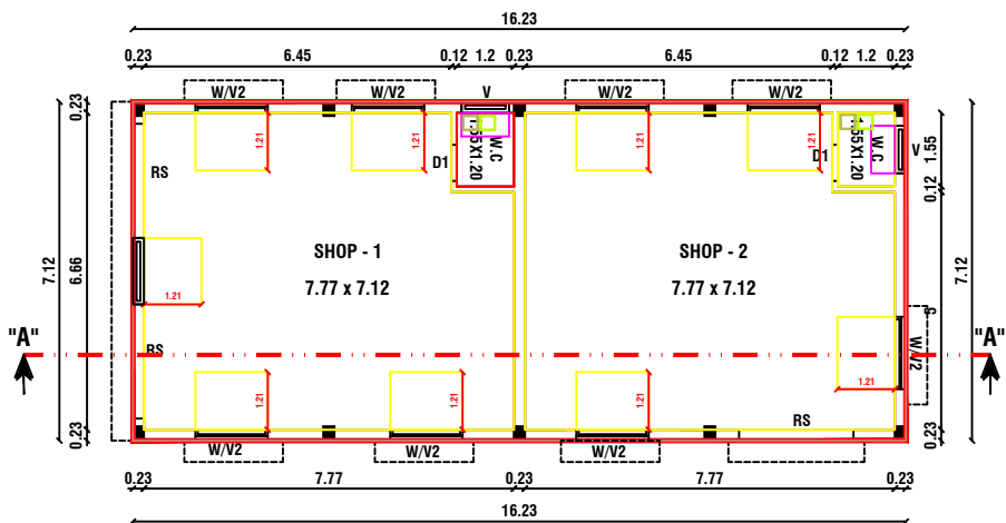
FLOOR - GROUND
