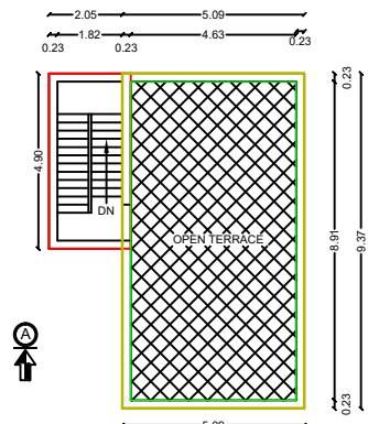
PLAN OF TERRACE FLOOR
