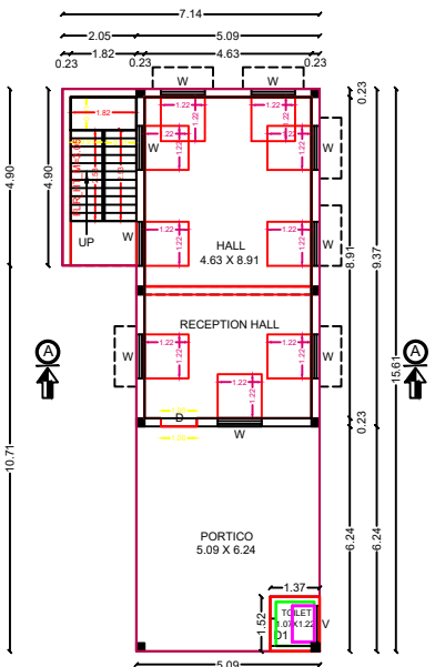
PLAN OF GROUND FLOOR
