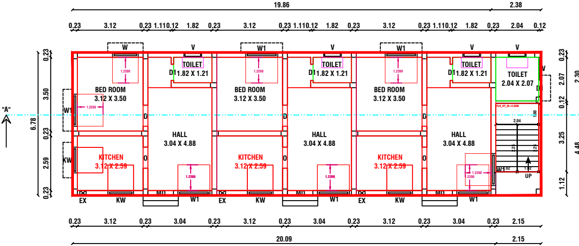
FLOOR - GROUND
