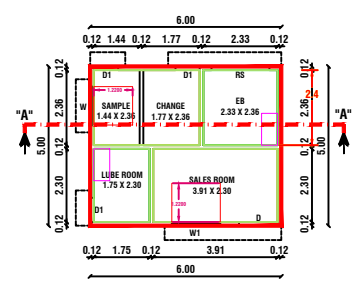
BLOCK - "A" FLOOR - GROUND PRO. GROUND FLOOR PLAN
