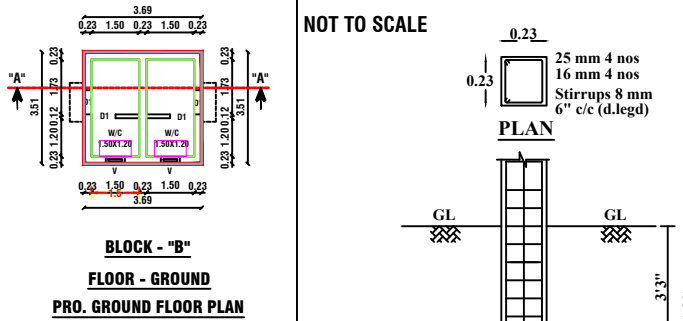
BLOCK - "B" FLOOR - GROUND PRO. GROUND FLOOR PLAN
