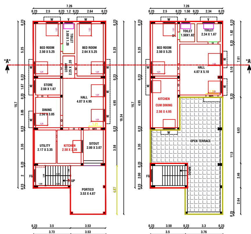
FLOOR - GROUND PRO. GROUND FLOOR PLAN
