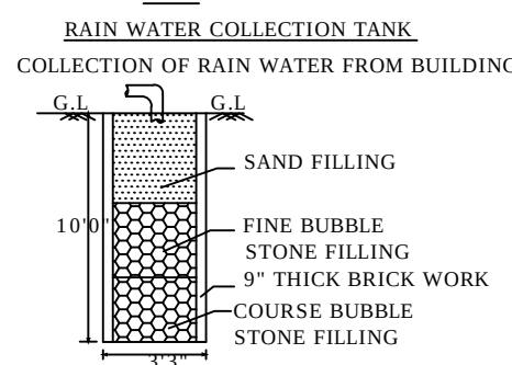
RAIN WATER COLLECTION TANK COLLECTION OF RAIN WATER FROM BUILDING
