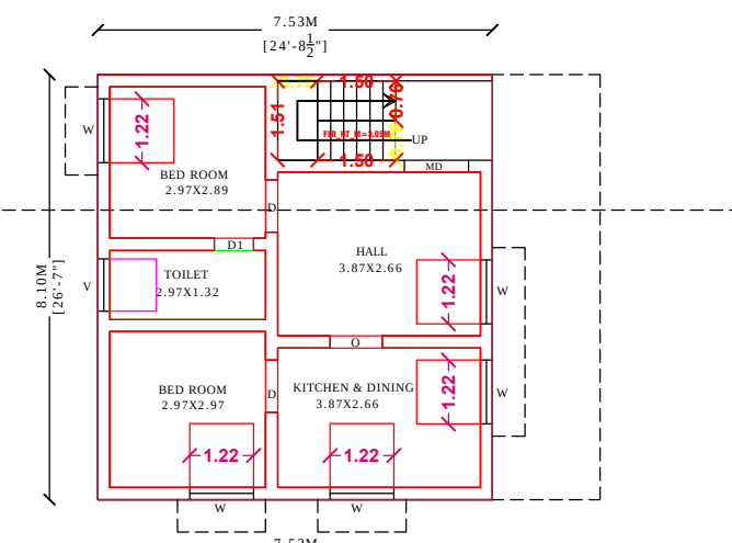
FLOOR - FIRST PRO. FIRST FLOOR PLAN
