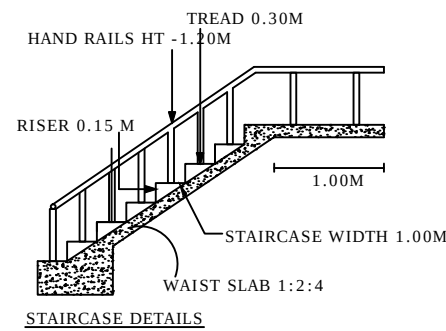
STAIRCASE DETAILS
