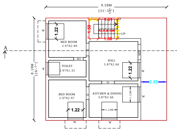
FLOOR - GROUND EXISTING. GROUND FLOOR PLAN
