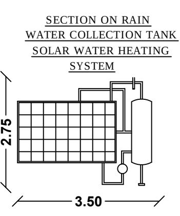
SECTION ON RAIN WATER COLLECTION TANK SOLAR WATER HEATING SYSTEM
