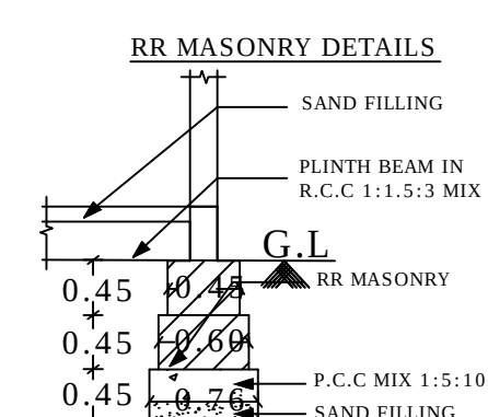
RR MASONRY DETAILS
