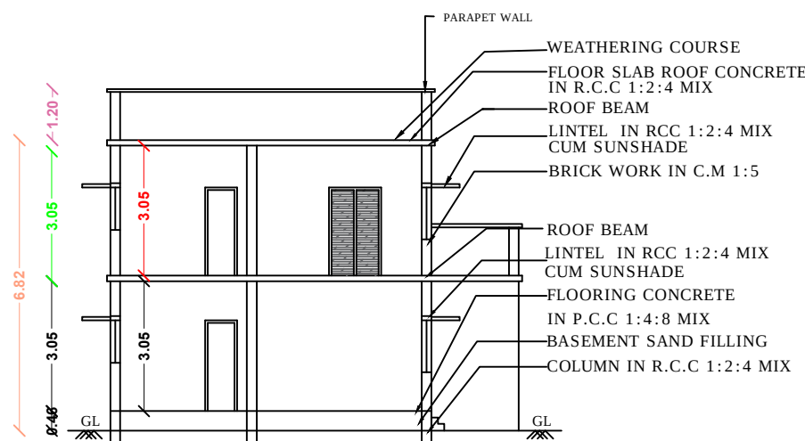
CROSS SECTION ON "A-A"
