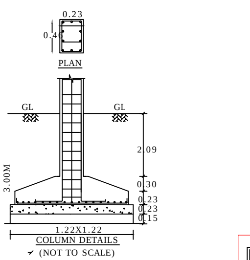
COLUMN DETAILS
