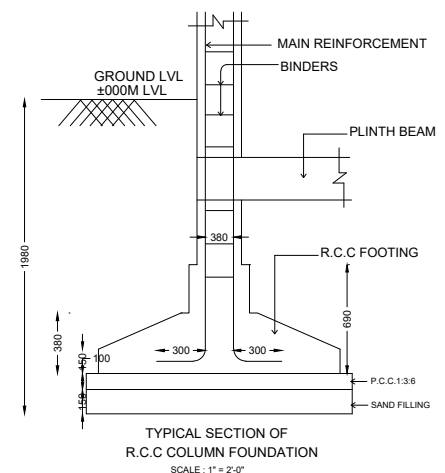
SECTION A - B
