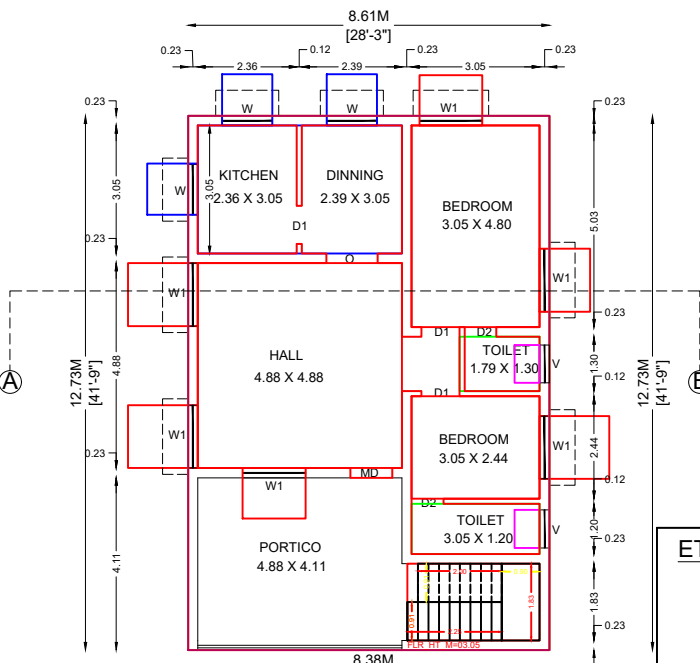
PROPOSED GROUND FLOOR PLAN (NORTH FACING)
