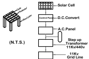
SOLAR SYSTEM FLOW DIAGRAM
