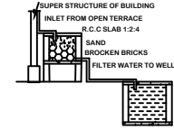
RAINWATER HARVESTING
