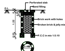
PERCOLATION PIT FOR 30 Sq. m. (Scale:- 1:50)
