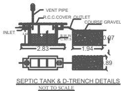
SEPTIC TANK & D-TRENCH DETAILS NOT TO SCALE
