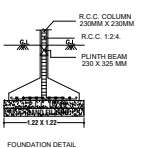
FOUNDATION DETAILS (NOT TO SCALE)
