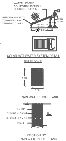
SECTION NO RAIN WATER COLL. TANK
