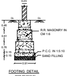
FOOTINGS DETAILS (NOT TO SCALE)
