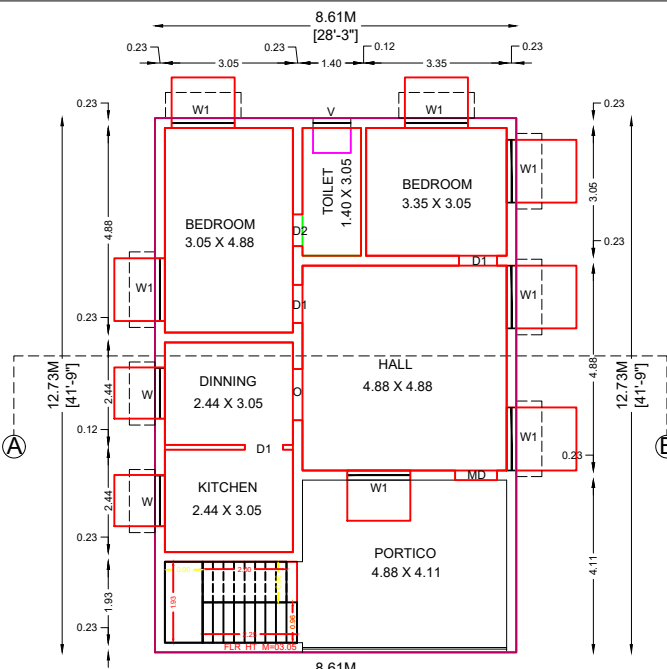
PROPOSED GROUND FLOOR PLAN (EAST FACING)
