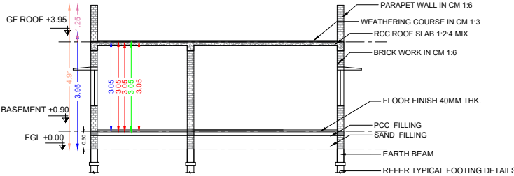
SECTION A - B
