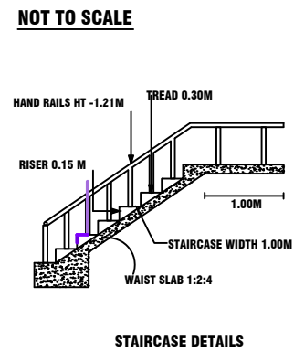
STAIRCASE DETAILS
