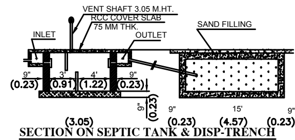
SECTION ON SEPTIC TANK & DISP-TRENCH
