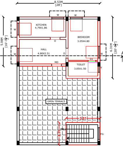
FLOOR - FIRST PRO. FIRST FLOOR PLAN
