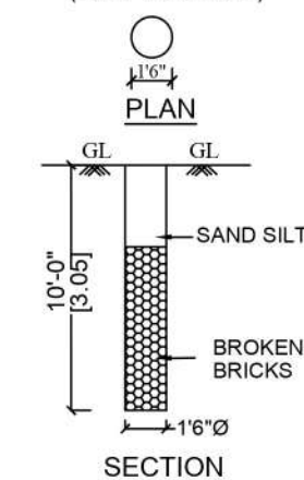
PERCOLATION PIT ( NOT TO SCALE)
