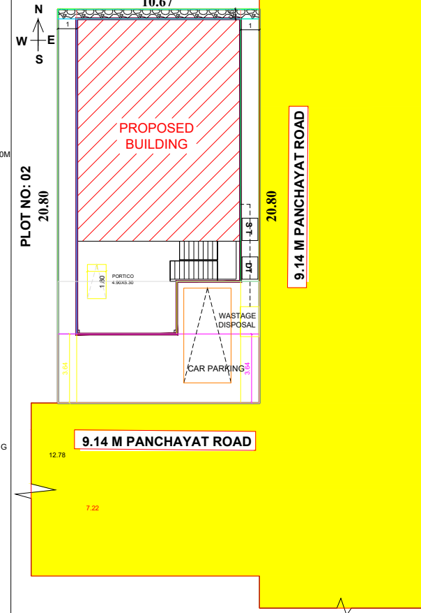
SITE PLAN: PROPOSED SCALE 1:100
