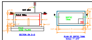
PLAN OF SEPTIC TANK SCALE 1"=2'-0"
