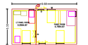
PRO.,GROUND FLOOR PLAN
