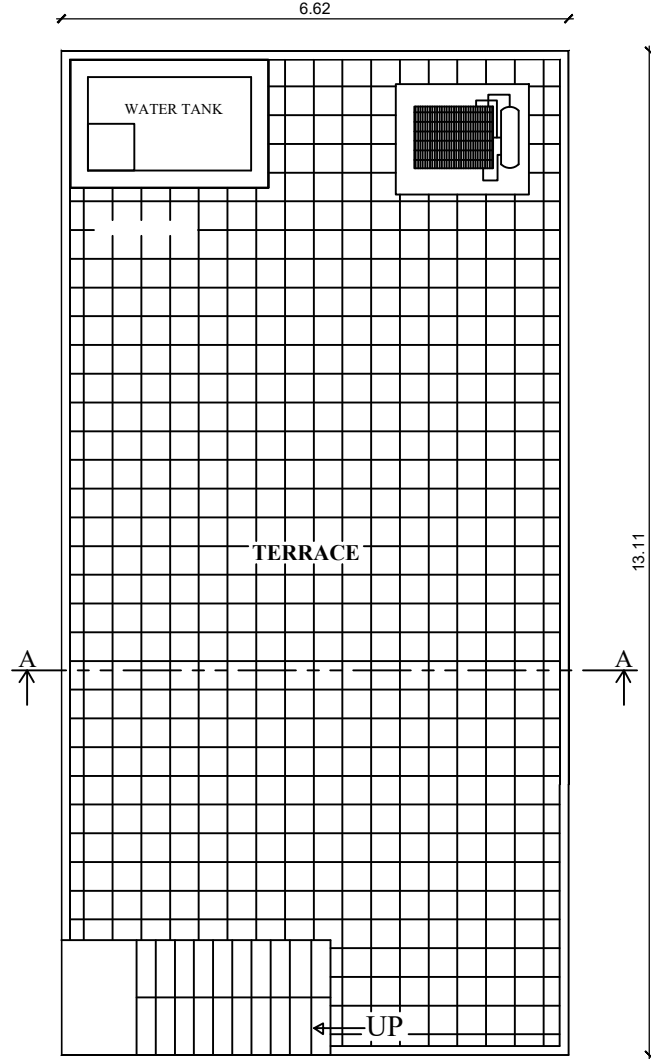
TERRACE PLAN
