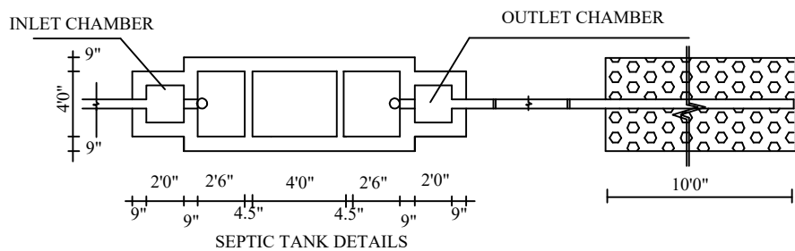
SEPTIC TANK DETAILS
