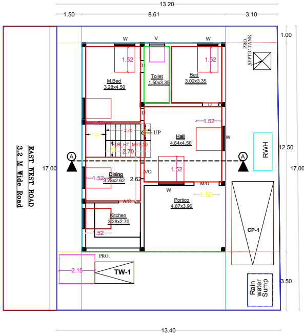
SITE PLAN CUM GROUND FLOOR PLAN
