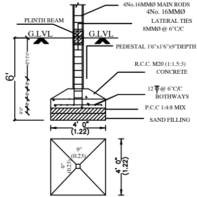
FOUNDATION DETAIL
