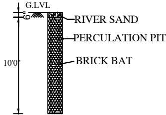
PERCOLATION PIT
