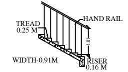
STAIRCASE DETAILS
