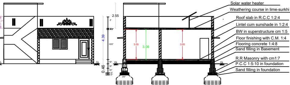
FRONT ELEVATION
