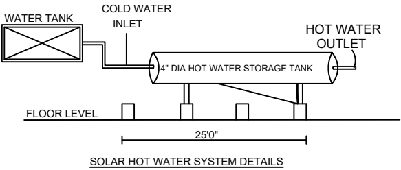
SOLAR HOT WATER SYSTEM DETAILS
