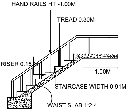
STAIRCASE DETAILS
