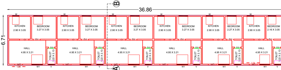
PROPOSED GROUND FLOOR PLAN (NORTH FACING)
