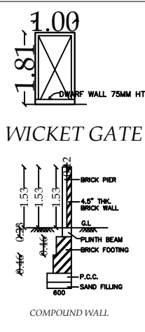
WICKET GATE DETAIL
