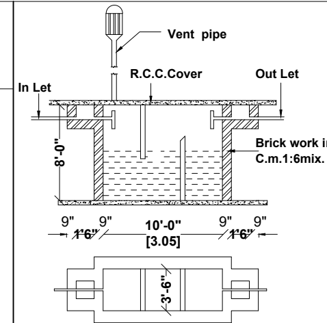
SEPTIC TANK DETAILS (NOT TO SCALE)
