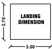
Physically Challenged Ramp landing
