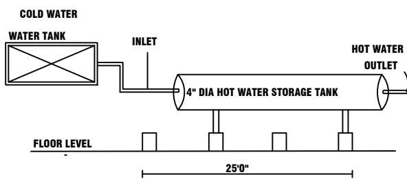
SOLAR HOT WATER SYSTEM DETAILS
