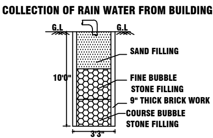
SECTION ON RAIN WATER COLLECTION TANK
