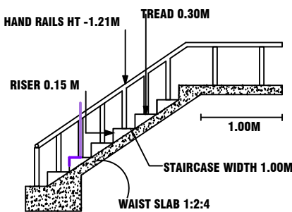
STAIRCASE DETAILS
