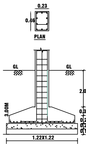
COLUMN DETAILS (NOT TO SCALE) (depends of soil condition)
