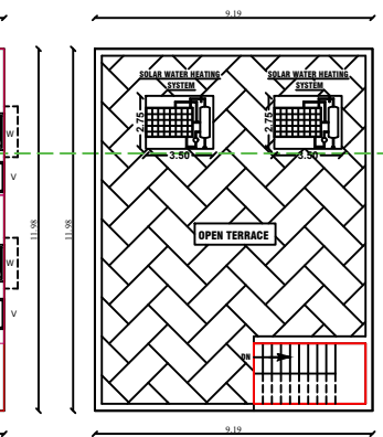
FLOOR-TERRACE PRO.TERRACE FLOOR PLAN
