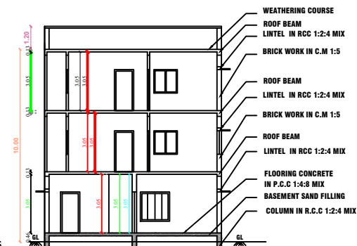
CROSS SECTION ON "A-A"
