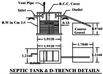
SEPTIC TANK & D-TRENCH DETAILS
