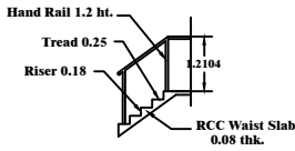
STAIRCASE DETAILS
