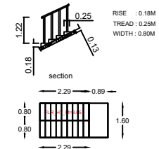
STAIRCASE DETAIL
