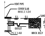
SECTION-AB
