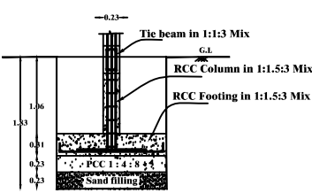
CROSS SECTION ON 'C - C'
