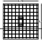
COLOUMN FOUNDATION DETAILS
