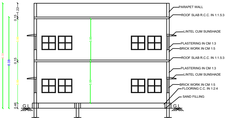
SECTION"A-B"
