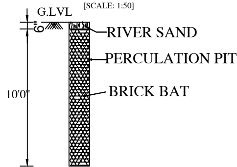
PERCOLATION PIT
